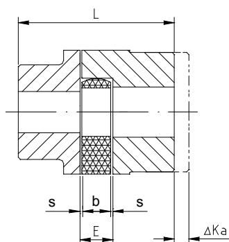
Axial Misalignment
